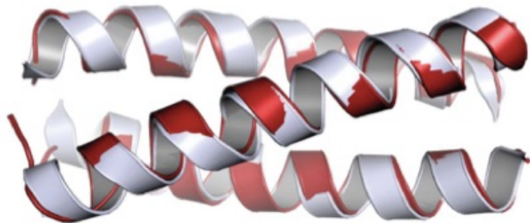
3v86 parallel trimer
